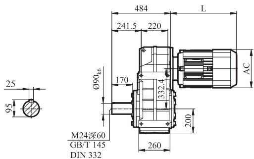
GFA/GFH/GFV107
