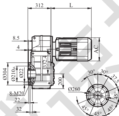
GFAF/GFHF/GFVF107
