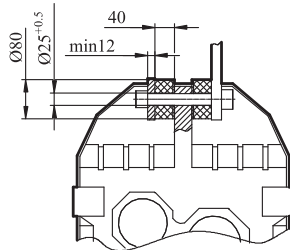
GFA107-T
